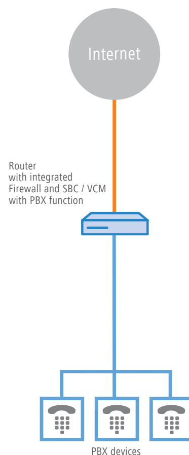
Fig. 4: Router with integrated firewall and SBC/VCM with PBX functions for small networks
